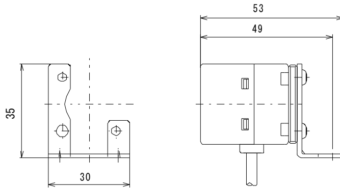
L type clamp (option)
